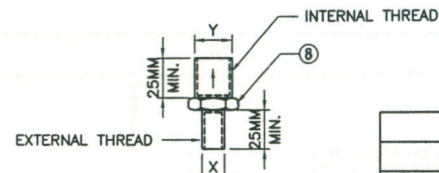
DETAIL-A (ADAPTOR)
